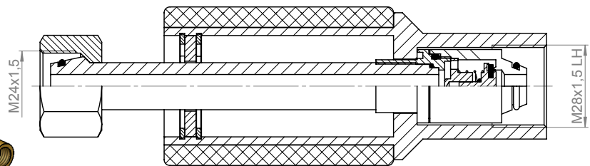
sectional drawing
